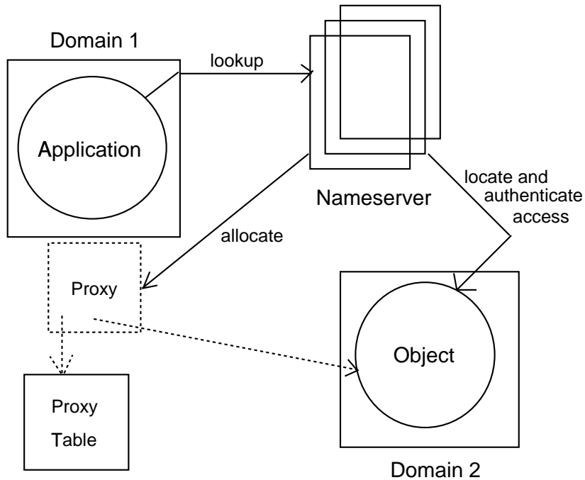
Figure 1: Object lookup
